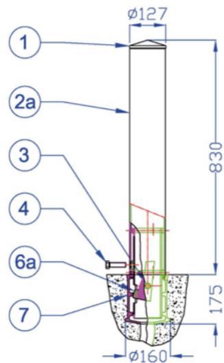
removable bollard
