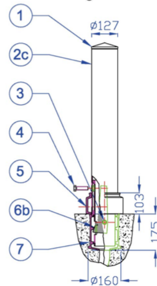
removable bollard with design base
